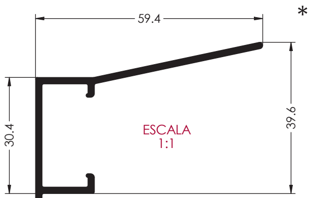
Ref. 2600 ALFEIZAR DE 60 mm
