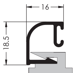
Ref. 1640 JUNQUILLO
