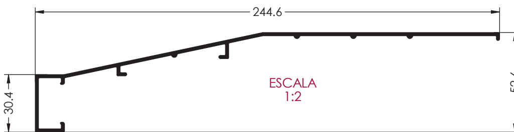
Ref. 2571 ALFEIZAR DE 245 mm
