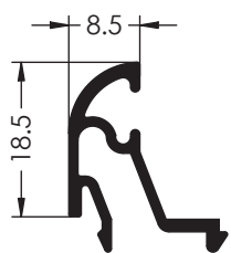
Ref. 1696 JUNQUILLO
