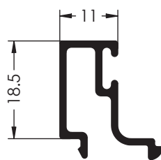
Ref. 1606 JUNQUILLO
