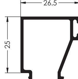
Ref. 9686 JUNQUILLO 25 mm
