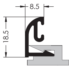
Ref. 1682 JUNQUILLO
