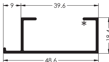
Ref. 2701 PREMARCO 49 mm
