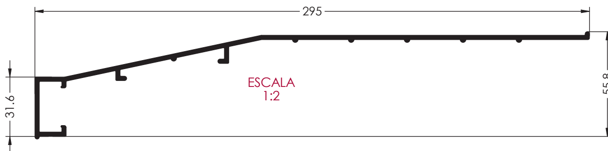
Ref. 2591 ALFEIZAR DE 295 mm
