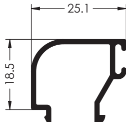
Ref. 1720 JUNQUILLO
