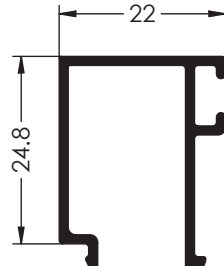
Ref. 1810 JUNQUILLO 25 mm
