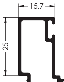
Ref. 1806 JUNQUILLO 25 mm
