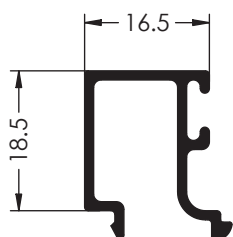
Ref. 1617 JUNQUILLO
