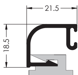
Ref. 1688 JUNQUILLO
