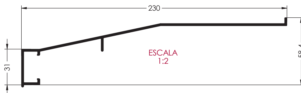
Ref. 2666 ALFEIZAR DE 230 mm
