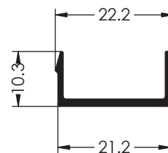
Ref. 1715 UNION CERCOS
