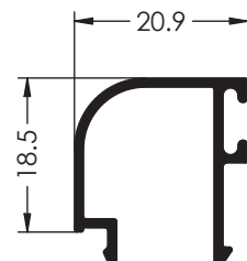
Ref. 1731 JUNQUILLO
