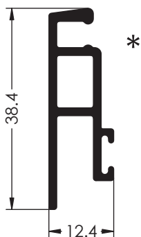
Ref. 9121 MOSQUITERA
