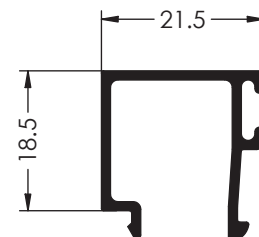
Ref. 1737 JUNQUILLO
