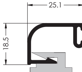
Ref. 1721 JUNQUILLO
