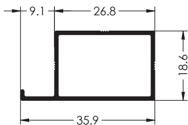
Ref. 2427 PREMARCO 36 mm
